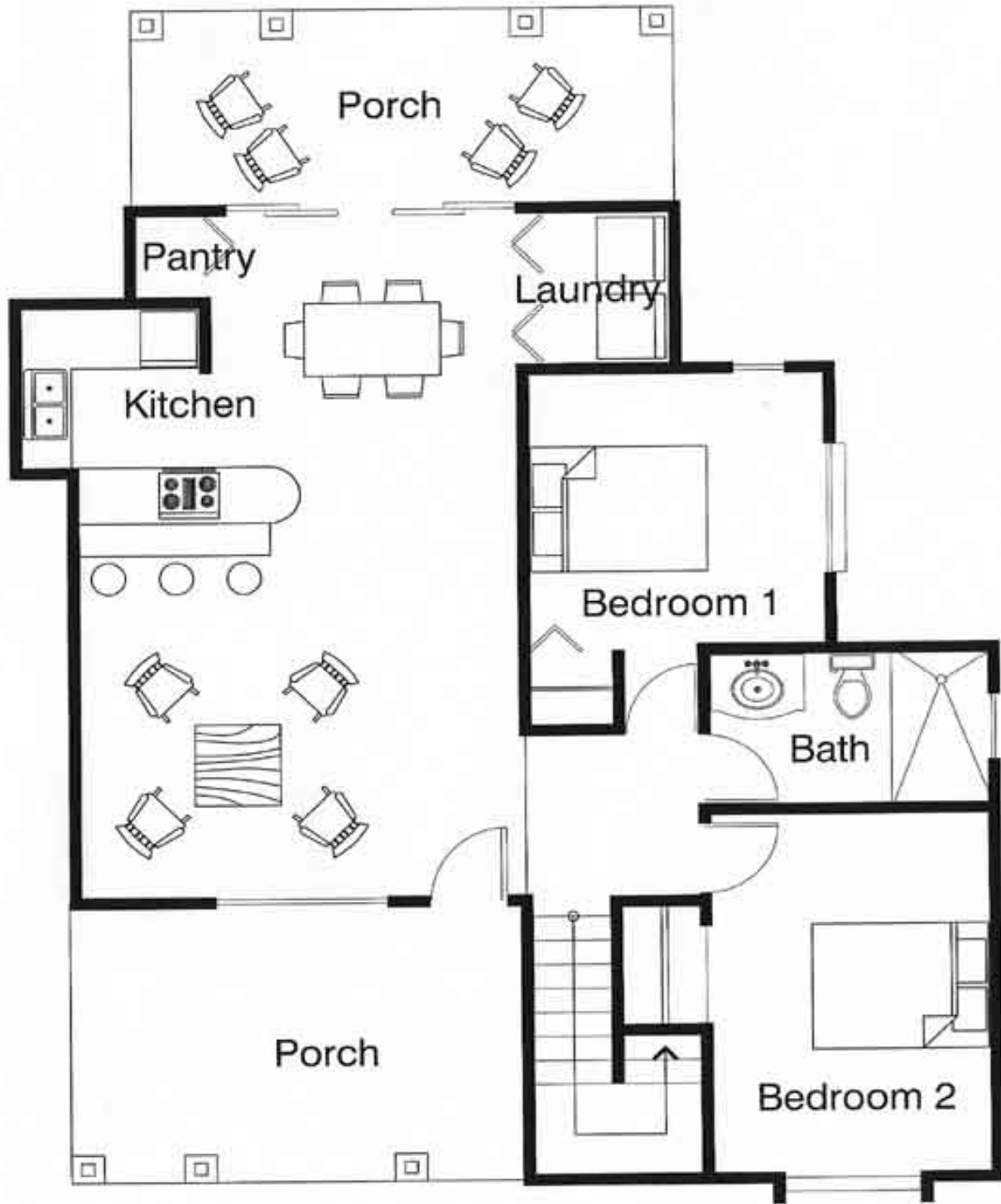
FIRST FLOOR
